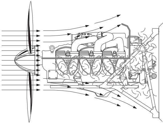
Figure 7. Airflow pattern over uncowled pressure cooled engine.
