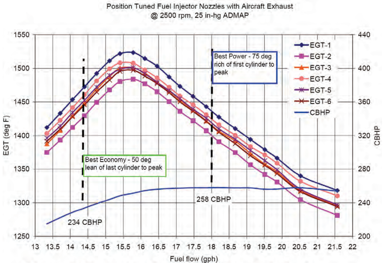
Figure 3. Engine Performance after Optimization
