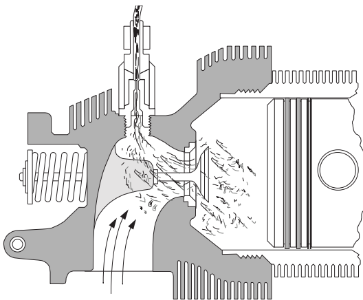
Figure 5. Fuel Injection Event
