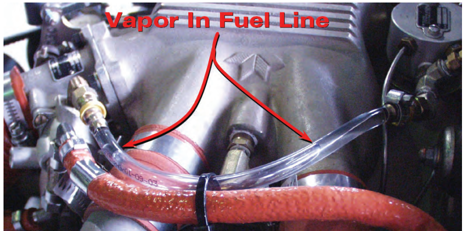
Figure 3. Heat Soaked Vapor in Clear Line
