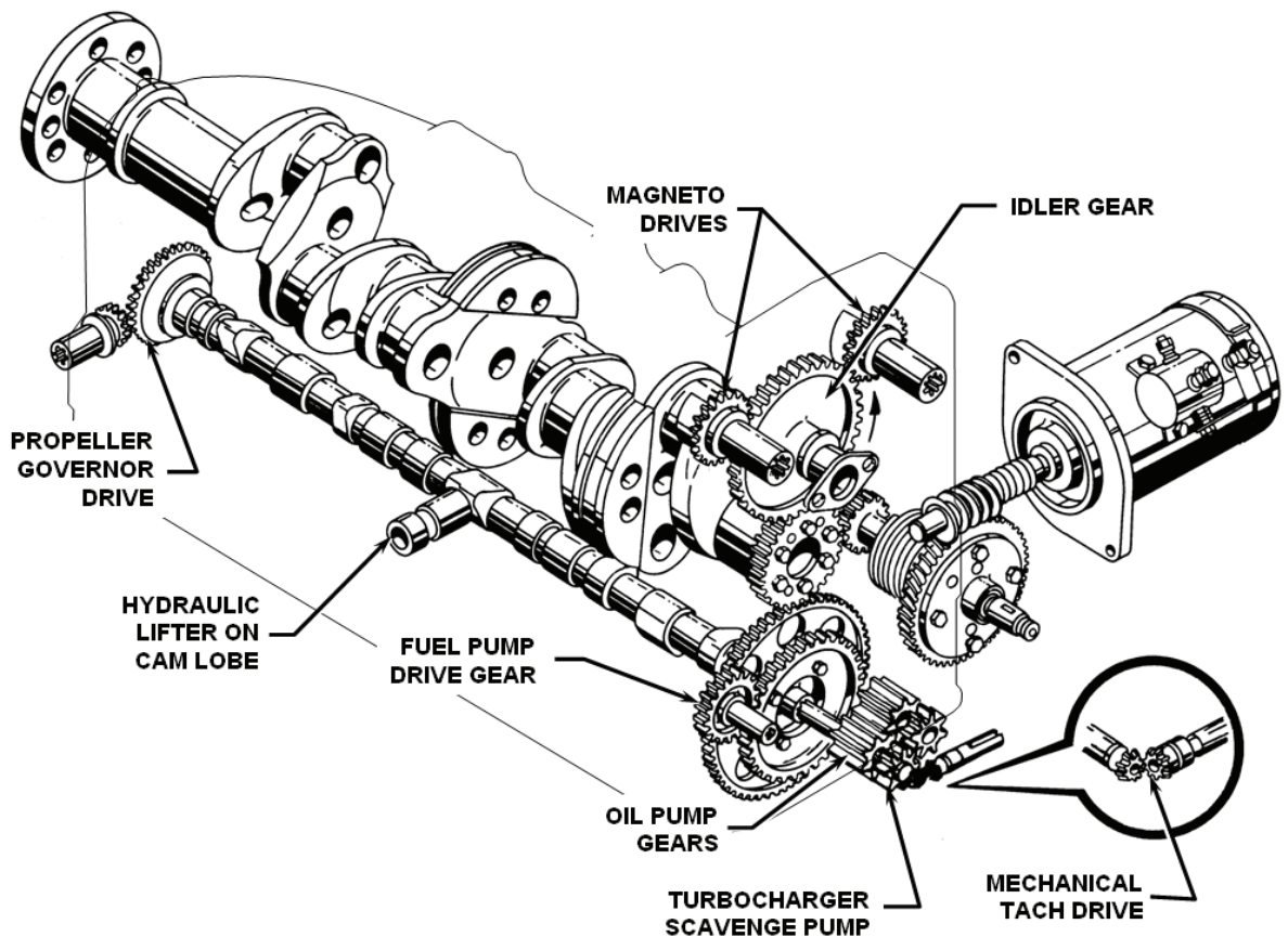
Typical Six Cylinder Gear Train Analysis Diagram
