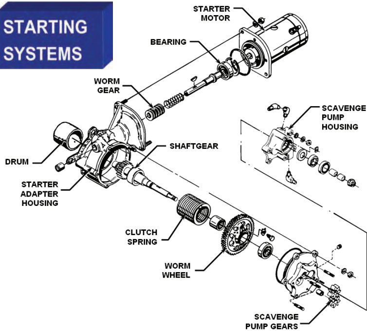
Starter Adapter with Turbo-Scavenge System
