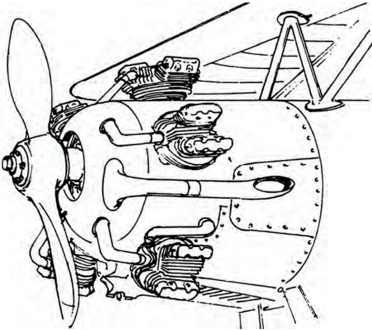
Figure 1. Velocity Cooling
