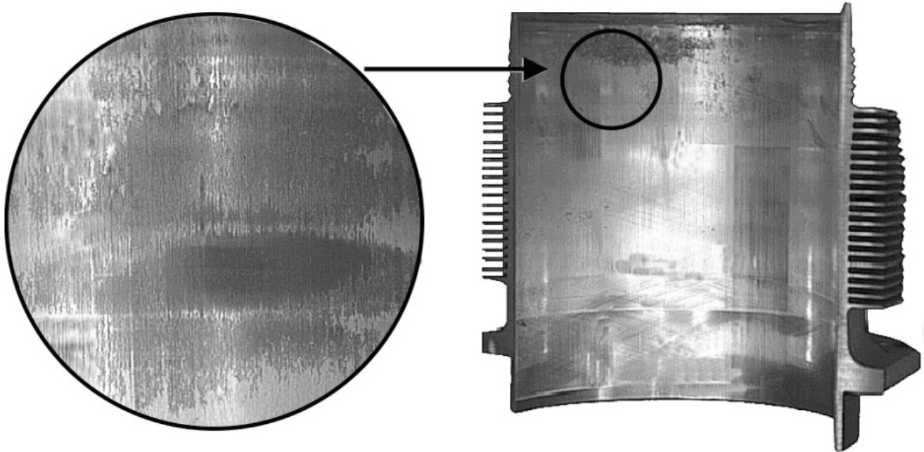
Figure 2. Heavy Rust Formation, Surface Pitting Has Altered Honed Pattern.
