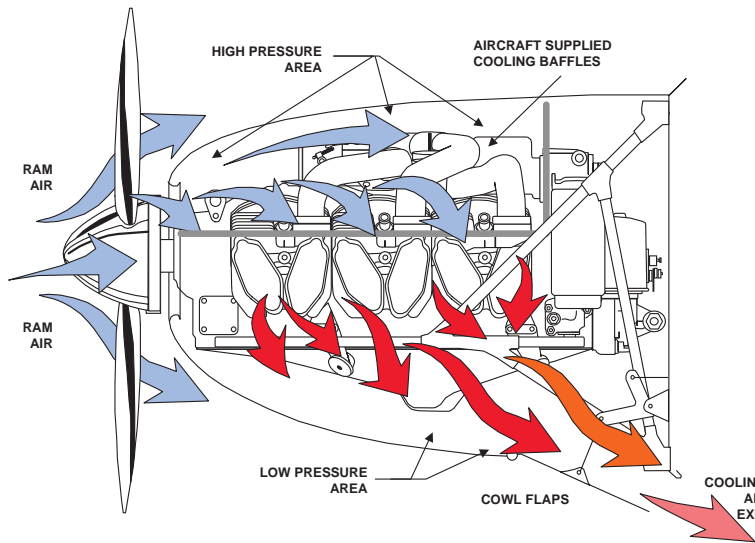
Figure 2. Desired Airflow
