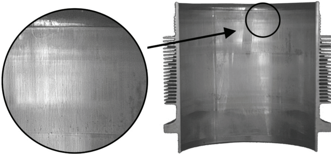
Figure 5. Heavily Worn Cylinder Bore
