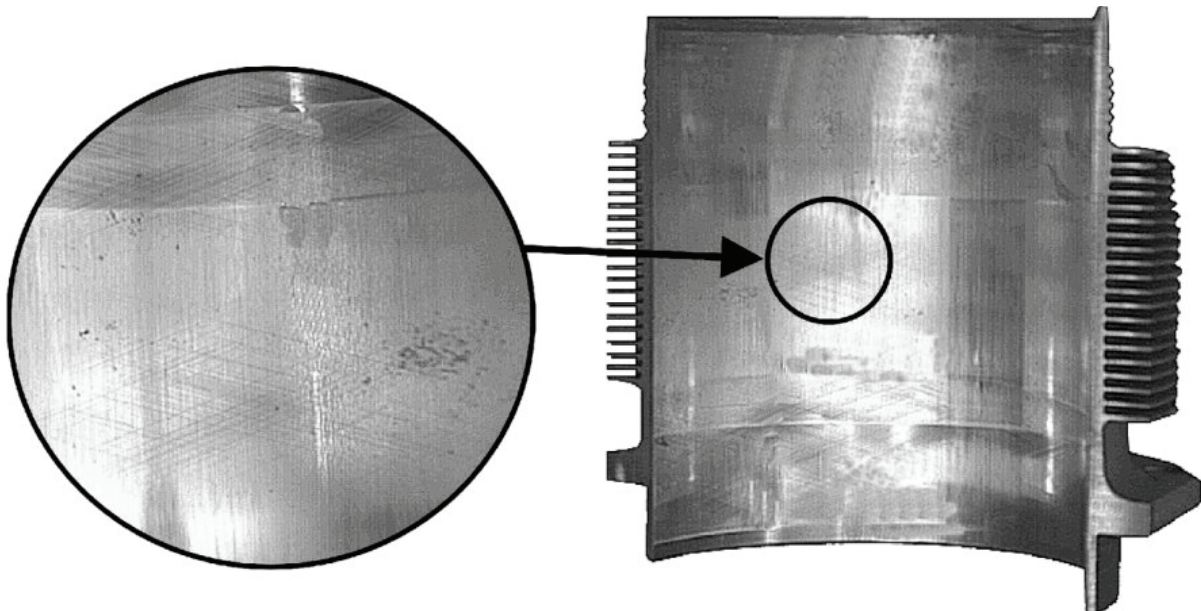
Figure 4. Typical Cylinder Bore At TBO
