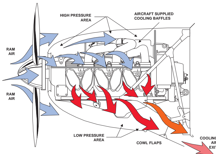
Figure 5. Properly directed airflow with precise baffle installation
