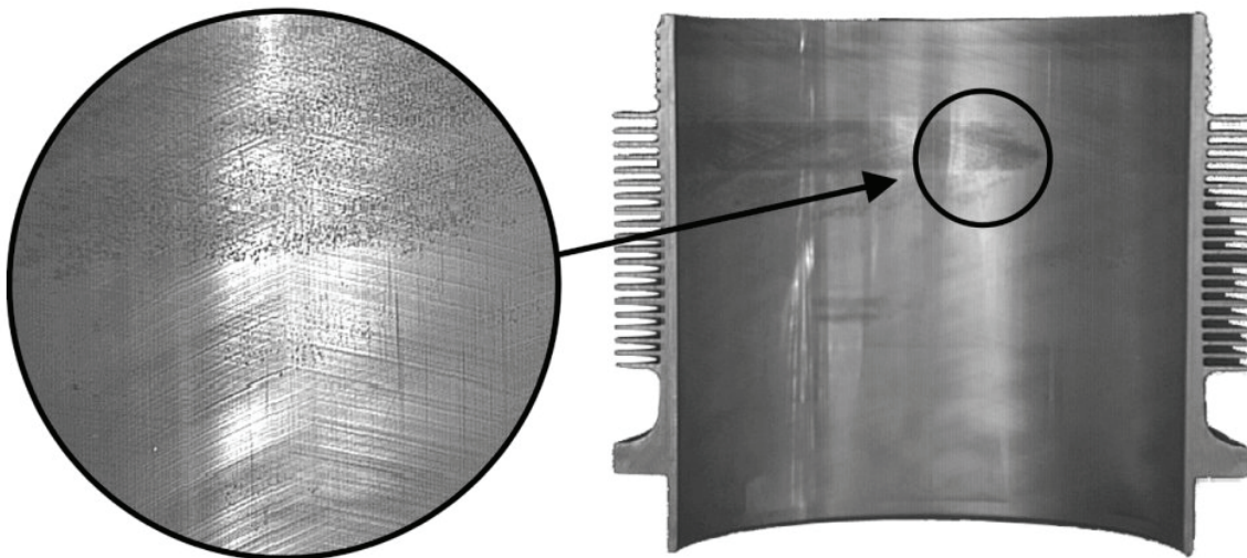
Figure 1. Light Rust Formation, Hone Not Affected.
