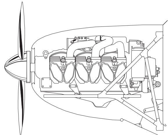
Figure 4. Typical Streamlined Installation of a Pressure Cooled Power Plant.
