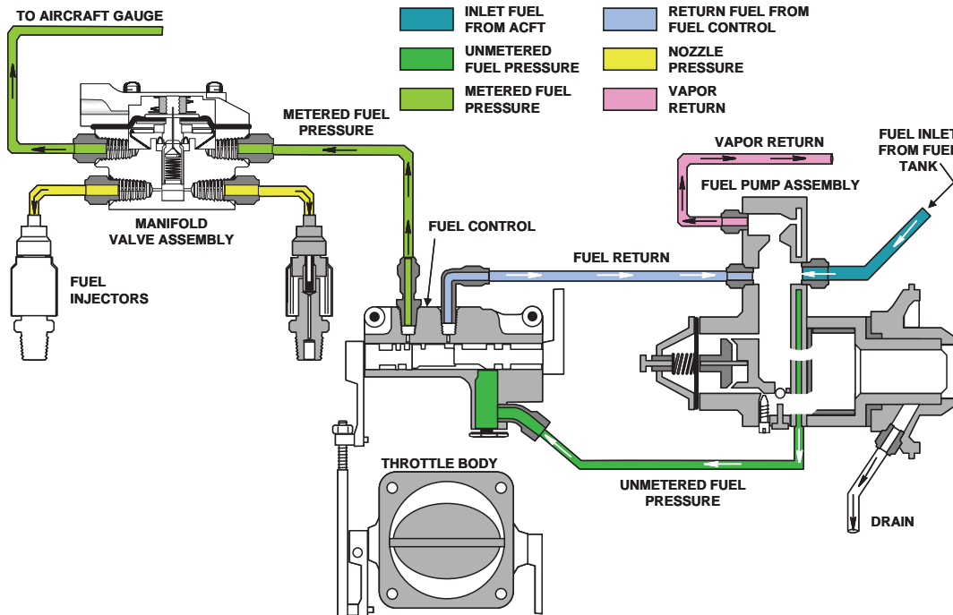
Typical Naturally Aspirated Fuel System Schematic
