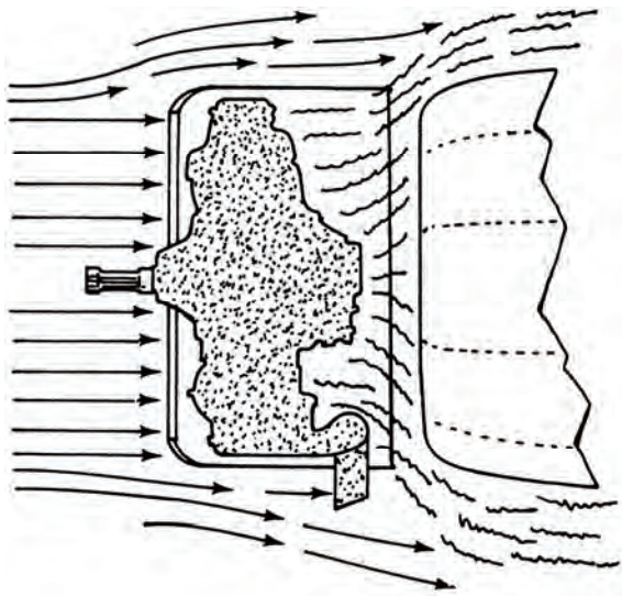
Figure 3. Early form of pressure cooling incorporating an NACA cowling.
