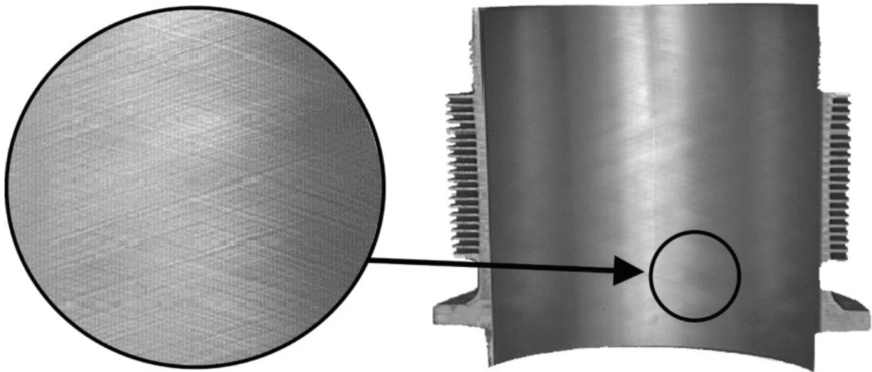
Figure 3. New Steel Cylinder Bore
